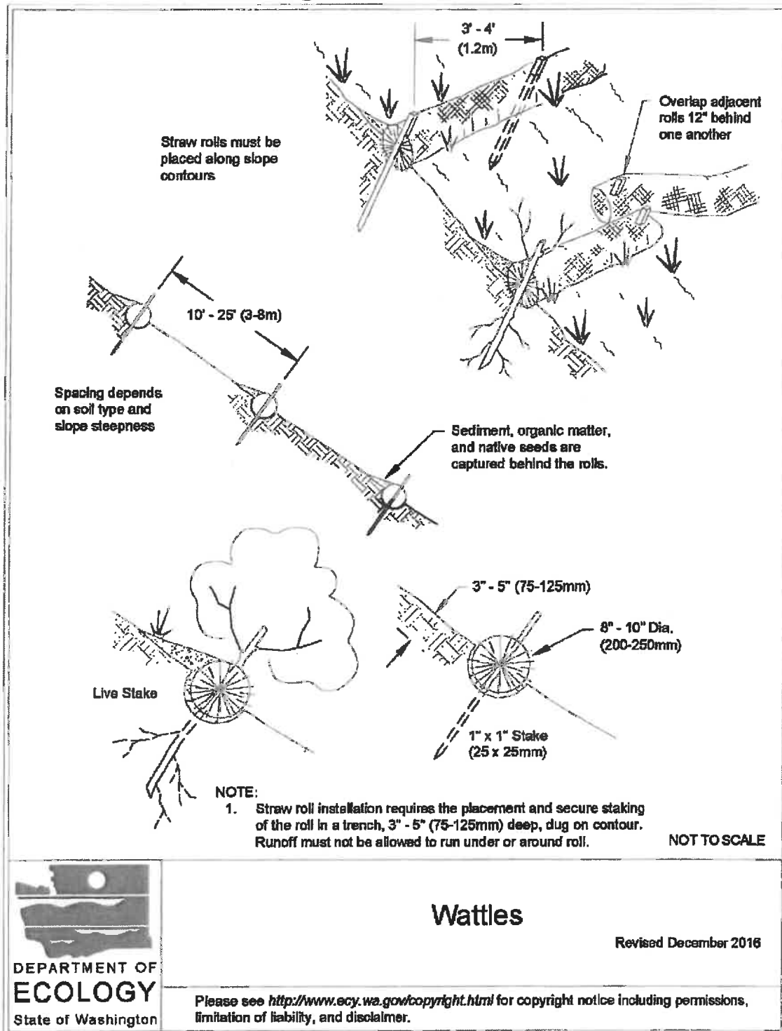
Figure II-3.24: Wattles
