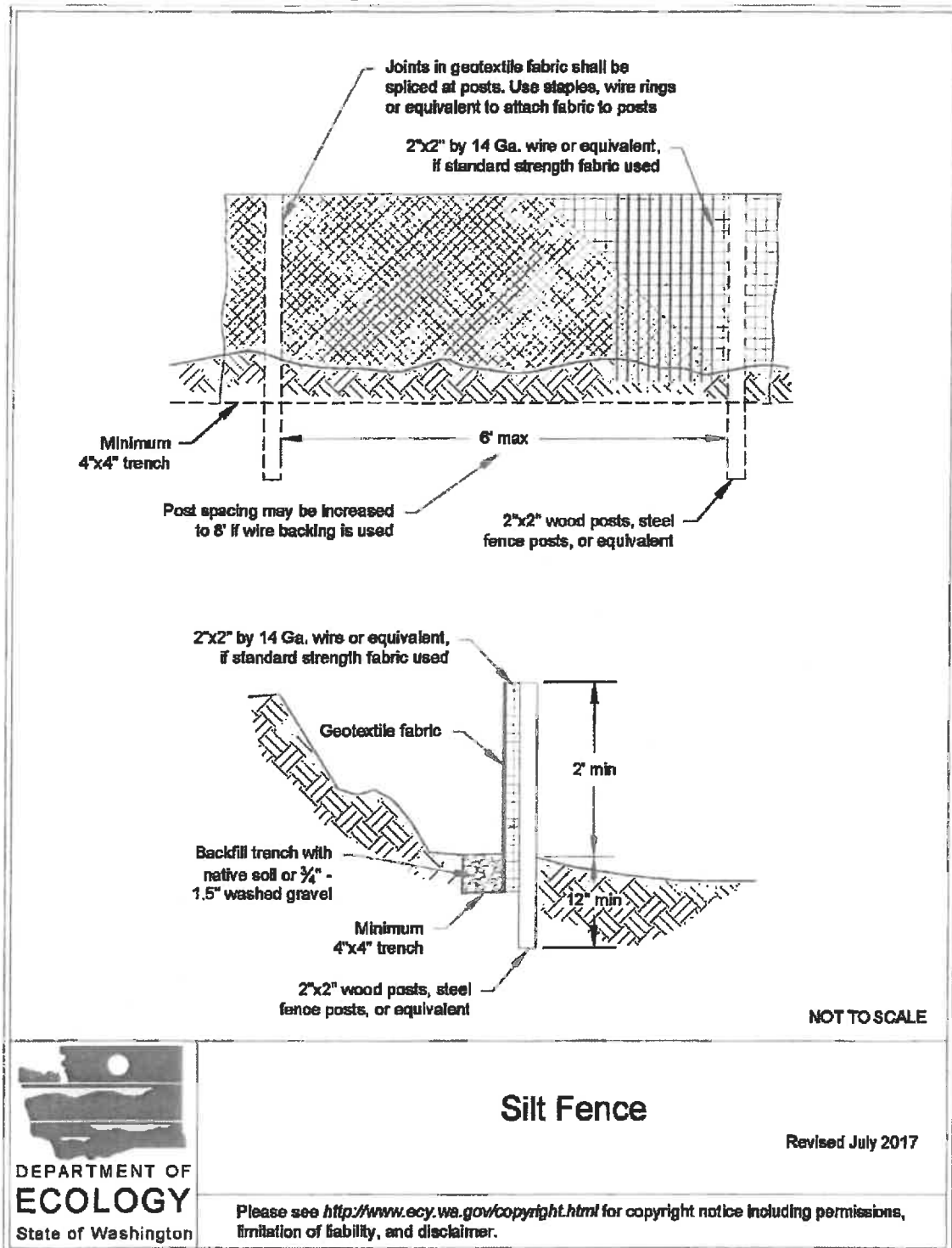
Figure II-3.22: Silt Fence
