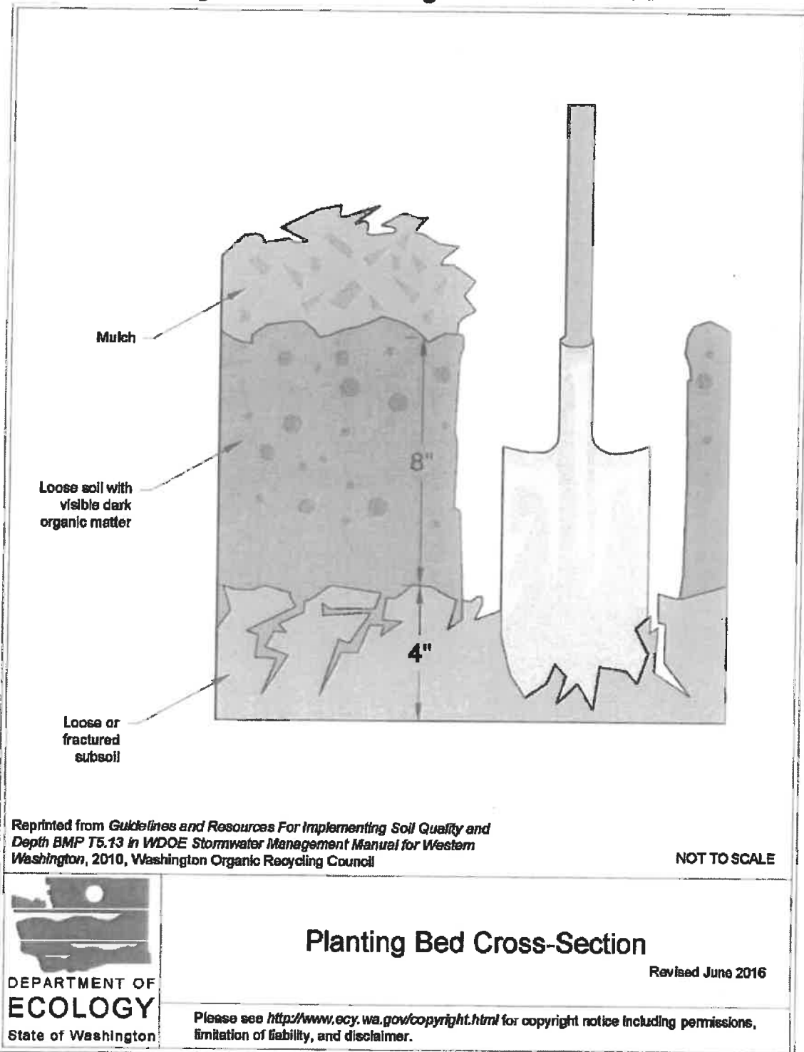
Figure V-11.1: Planting Bed Cross-Section
